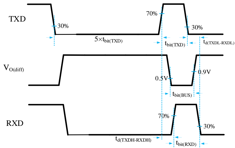
Fig 12 CAN FD timing definitions according to ISO 11898-2:2016
