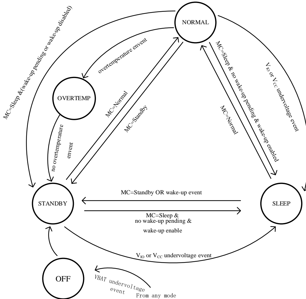
Fig 3 system controller state diagram
