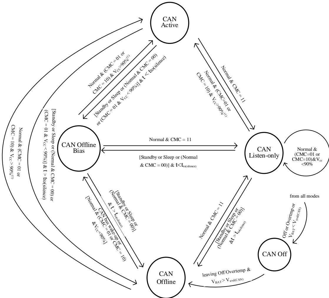
Fig 4 CAN transceiver state machine
