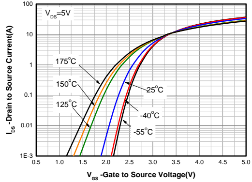
Transfer Characteristics (4)
