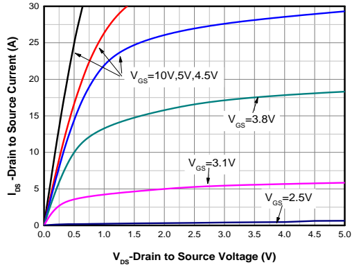
Output Characteristics (4)
