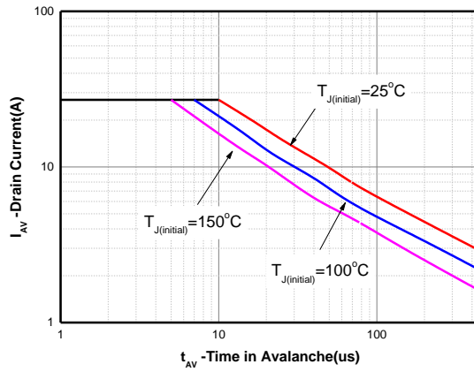
Avalanche characteristics
