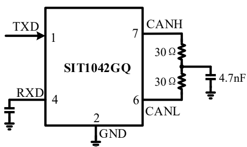
Figure 5 Transceiver bus symmetry test circuit
