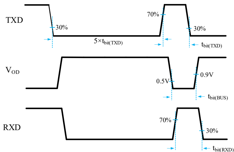
Figure 2 t_{bit} delay
