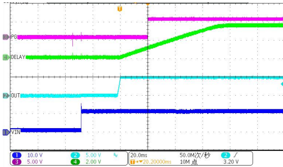
PG VS POWER UP@ Vin=12V, Vout=5V, IOUT=300mA, CDELAY=100 nF
