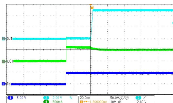
EN=L→H @ Vin=12V, Vout=5V, IOUT=500mA
