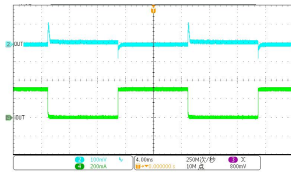
iOUT=1 &lt;-&gt; 300mA @ Vin=12V, Vout=5V
