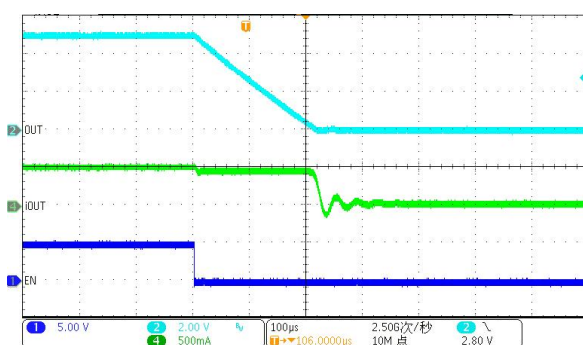
EN=H→L @ Vin=12V, Vout=5V, IOUT=500mA
