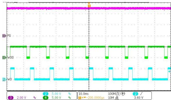
Fault (over maximum open-window duration t(WD) / 2 )
