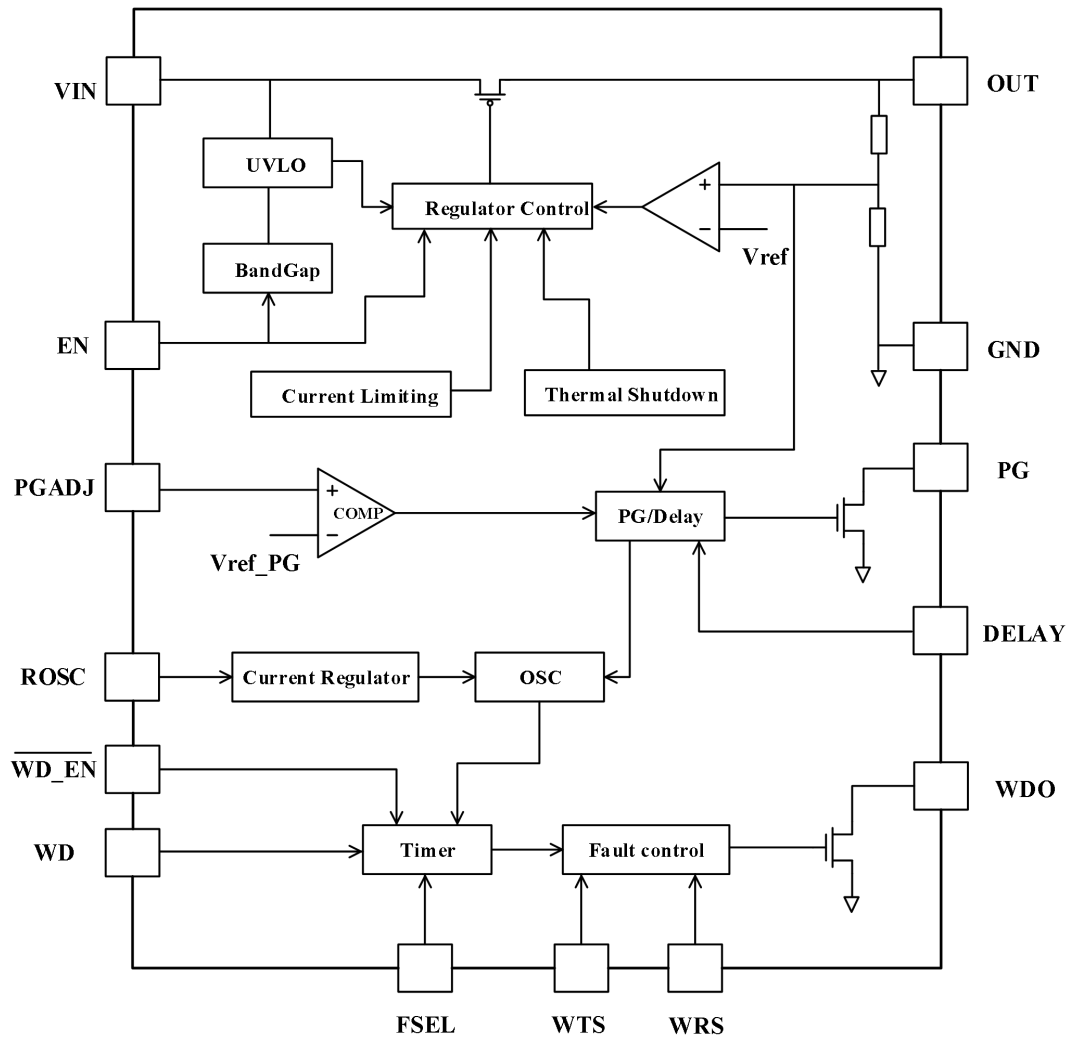
Figure 2 Internal block diagram of SIT24XX5Q series
