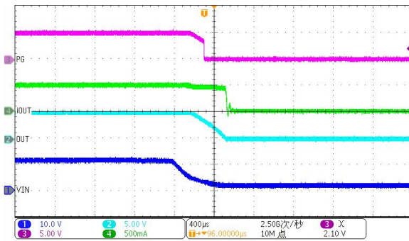
Power-OFF @ Vin=12V, Vout=5V, IOU=500mA
