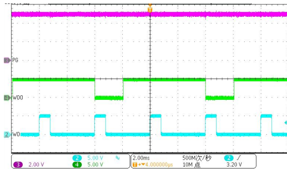
Fault (Receiving a WD rising edge during the closed window)
