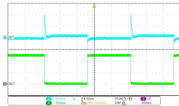
iOUT = 1 &lt;-&gt; 500mA @ Vin=12V, Vout=5V
