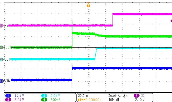
Power-Up @ Vin=VEN=12V, Vout=5V, IOU=500mA
