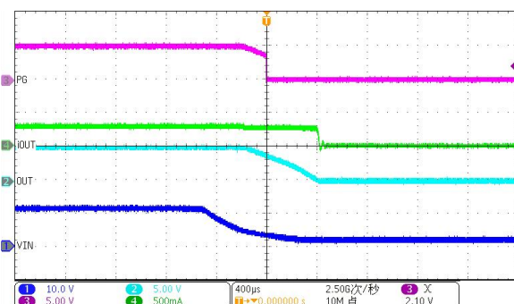
Power-Up @ Vin=VEN=12V, Vout=5V,
