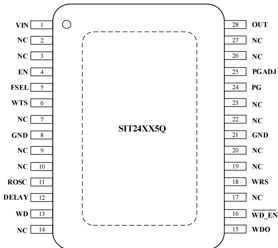
Figure 1 SIT24XX5Q Pin configuration
