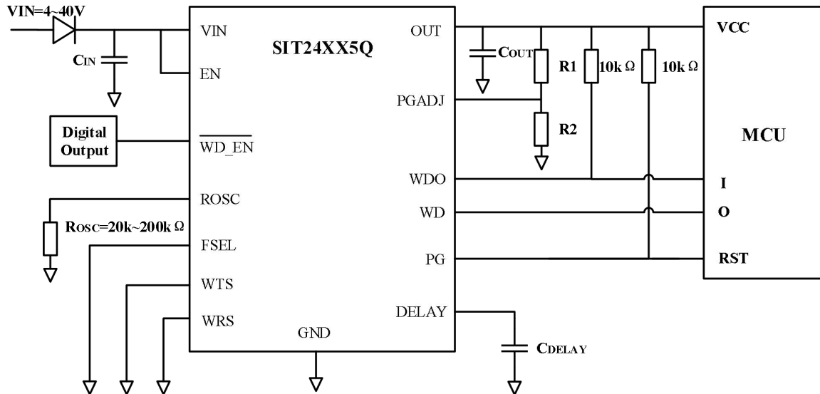
Figure 3 SIT24XX5Q series typical application diagram
