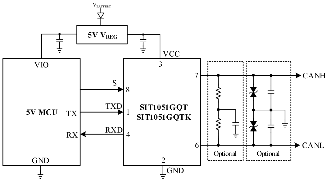
Figure 6 SIT1051GQT, SIT1051GQTK and 5V MCU typical application diagram
