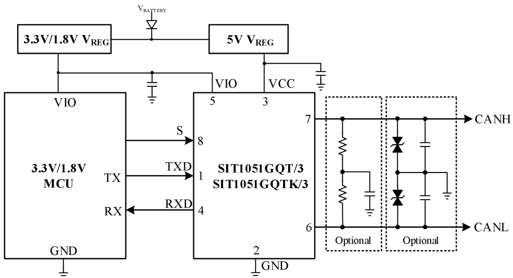
Figure 7 SIT1051GQT/3, SIT1051GQTK/3 and 1.8V/3.3V MCU typical application diagram
