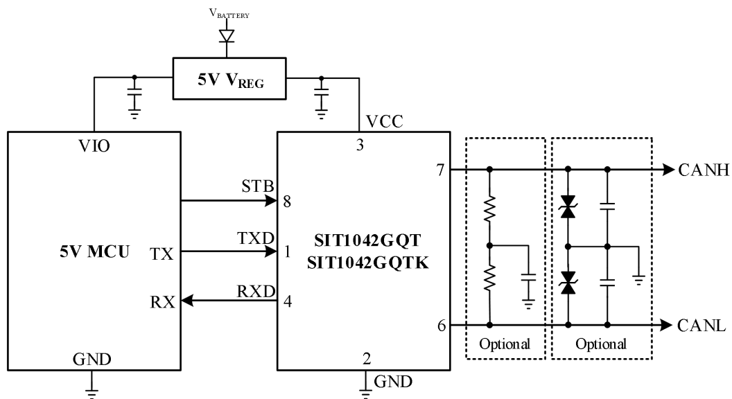
Figure 6 SIT1042GQT, SIT1042GQTK and 5V MCU typical application diagram
