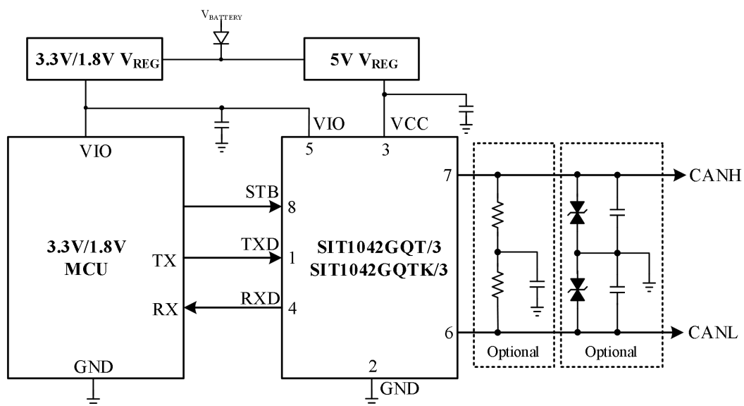
Figure 7 SIT1042GQT/3, SIT1042GQTK/3 and 1.8V/3.3V MCU typical application diagram
