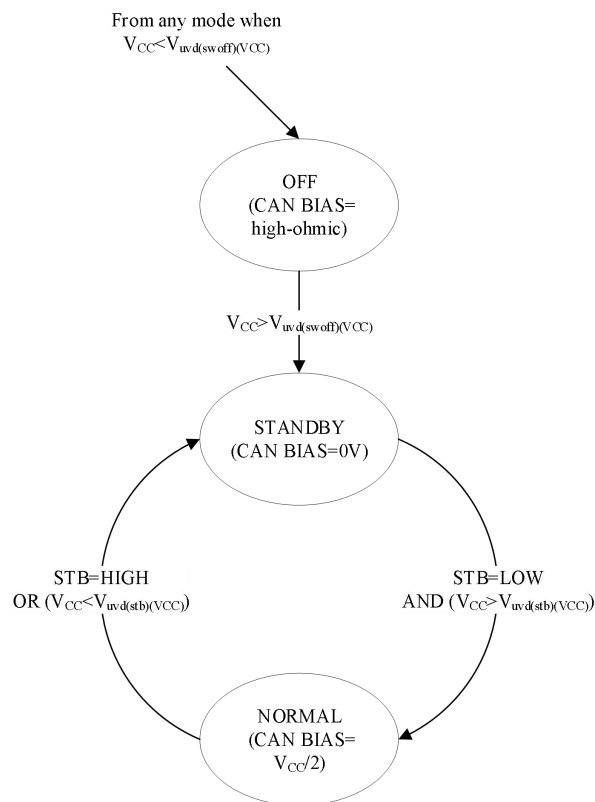
Figure 8 SIT1044G state diagram
