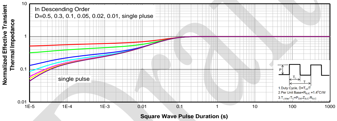
Transient Thermal Response (Junction-to-Case)
