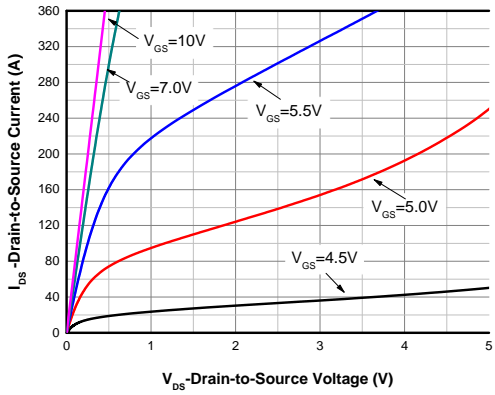
Output Characteristics (4)
