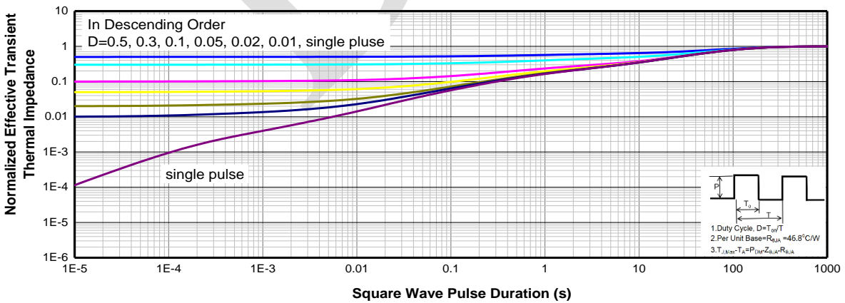
Transient Thermal Response (Junction-to-Ambient)
