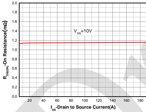
On-Resistance vs. Drain Current (4)
