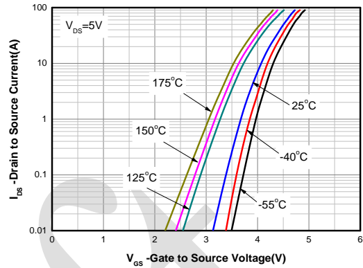
Transfer Characteristics (4)
